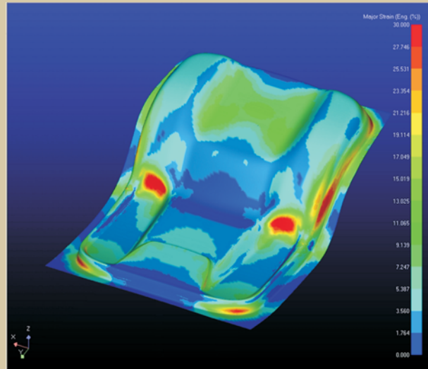
Complete incremental analysis solution in the proven FormingSuite environment
