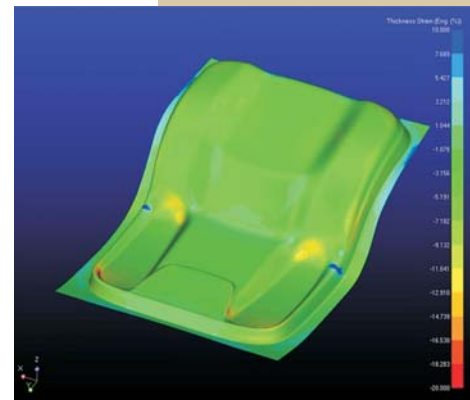
A complete set of results visualization tools help identify formability issues
