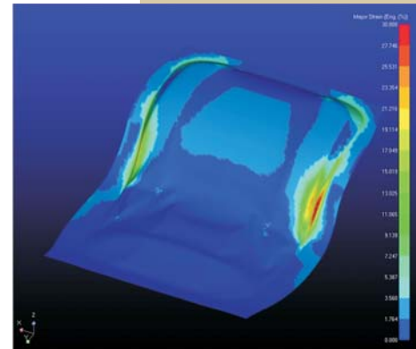
Panel breakdown feature provides results throughout forming operation
