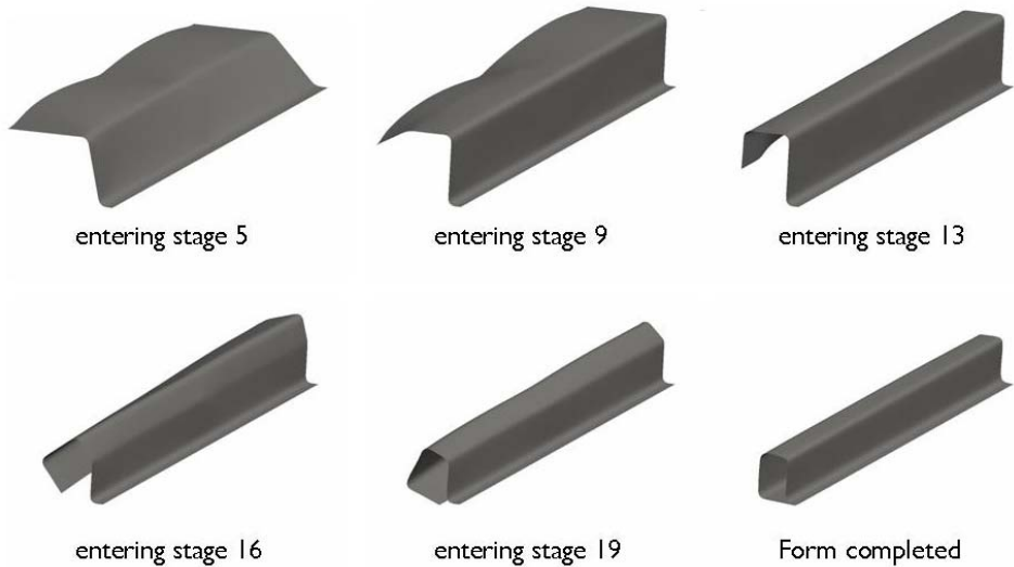
Figure 4: Roll forming simulation
