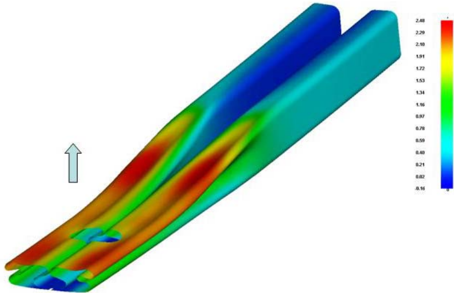
Figure 6: Crushed beam showing vertical springback post-crushing operation
